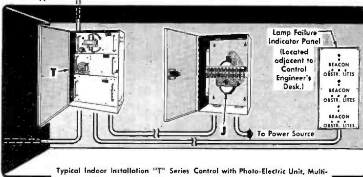
Typical Tower Lighting Installation (Conduit Kit—Triangular Tower)
